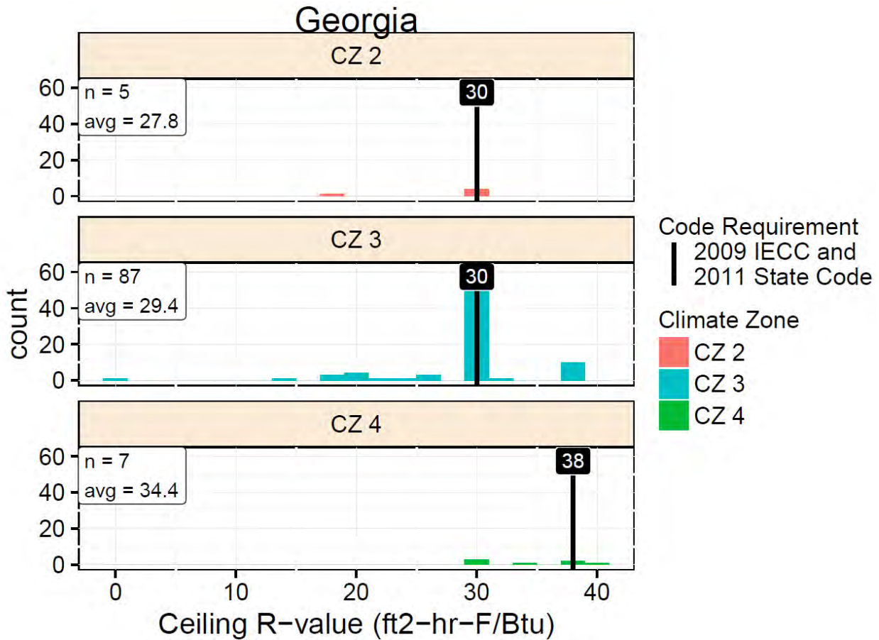
Figure 3.8. Ceiling R-Value
