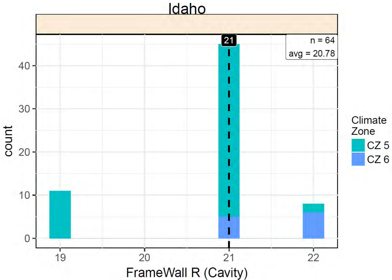
Figure 3.4. Wall R-Values
